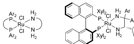
Scheme 1. General structure of Noyori catalysts and the most selective catalyst known
