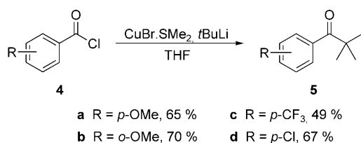
Scheme 3. Preparation of tert -butyl ketones.
