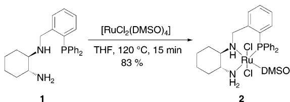
Scheme 2. Synthesis of the ruthenium catalyst 2 .
